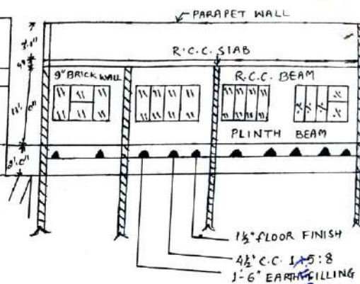
SECTION AT X-Y
